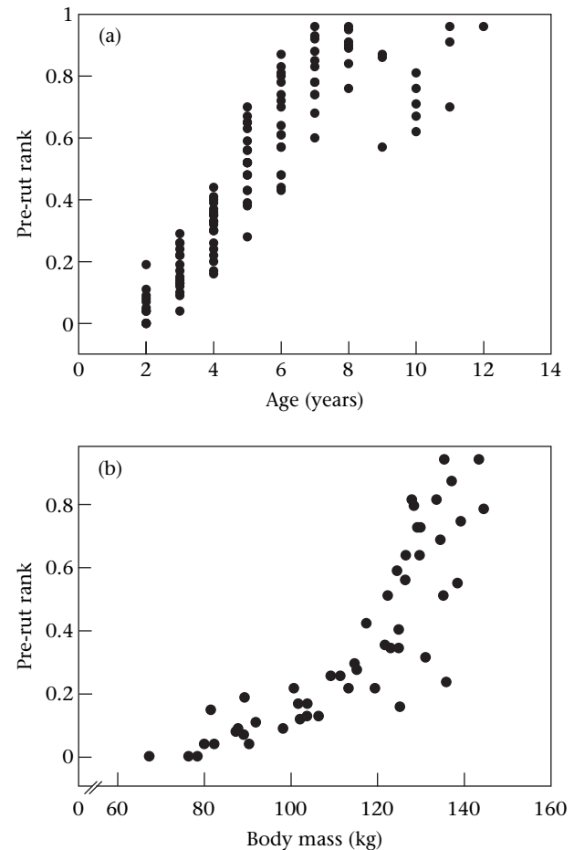
Figure 3. (a) Relationship between age and social rank for bighorn rams aged 2 years and older. A linear mixed model explained 86% of the variance (age: F_{1,64} = 558.54 , N = 119 observations from 53 individuals, P < 0.001 ; age 2 : F_{1,64} = 61.02 , P < 0.001 ). (b) Relation between body mass in early autumn and social rank for bighorn rams aged 2 years and older. A linear mixed model explained 73% of variance (mass: F_{1,23} = 118.61 , N = 51 observations from 26 individuals, P < 0.001 ; mass 2 : F_{1,23} = 7.85 , P = 0.01 ).
